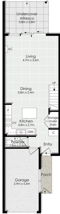
Ground Floor
