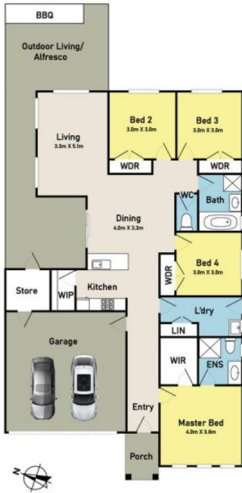
Floor Plan
