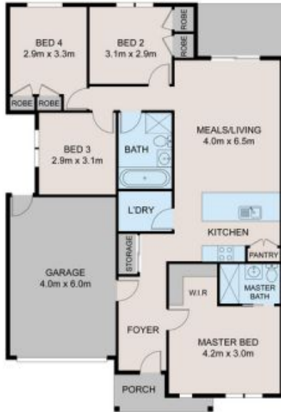
FLOOR PLAN
