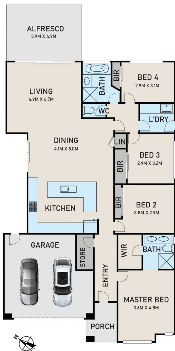
FLOOR PLAN
