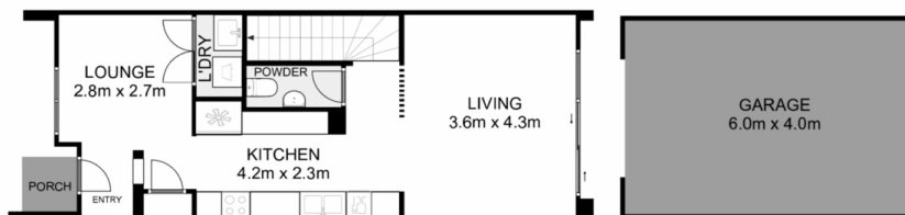
GROUND FLOOR
