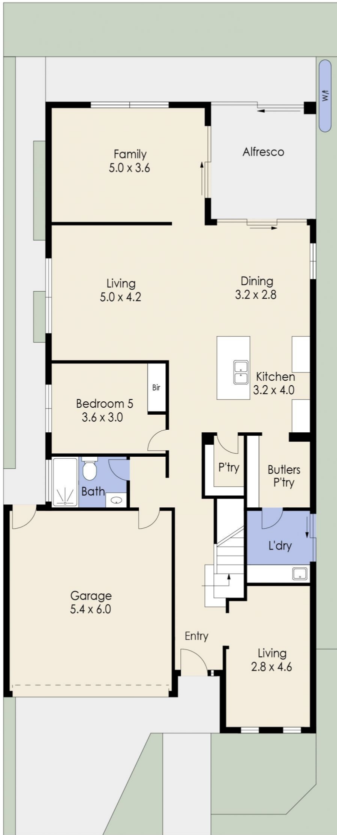
Ground Floor
