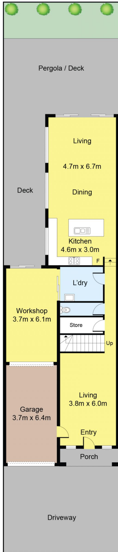
Ground Floor
