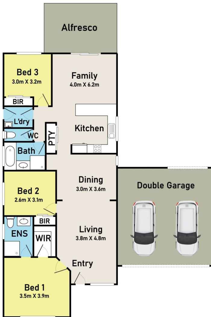
Floor Plan
