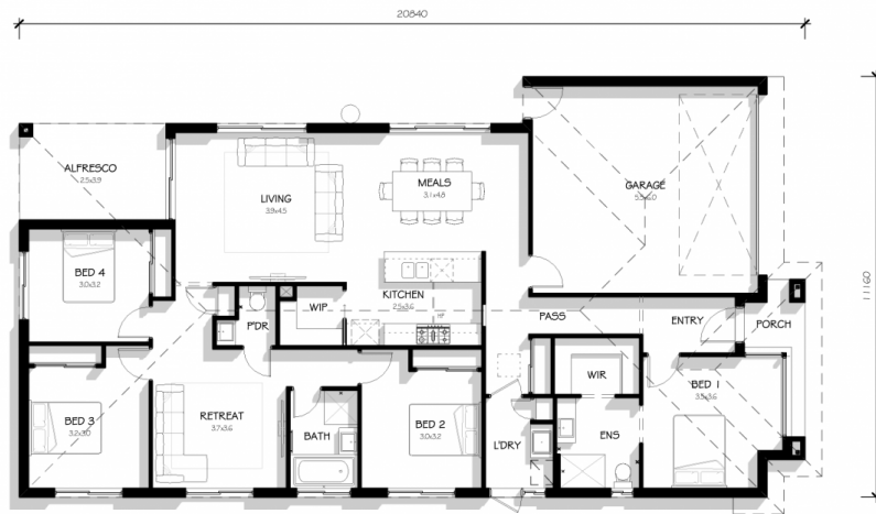
1 FLOOR PLAN - MARKETING 1 : 100
